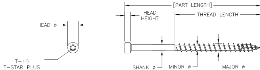
FIGURE 1. SPAX® XTT08 FASTENER
