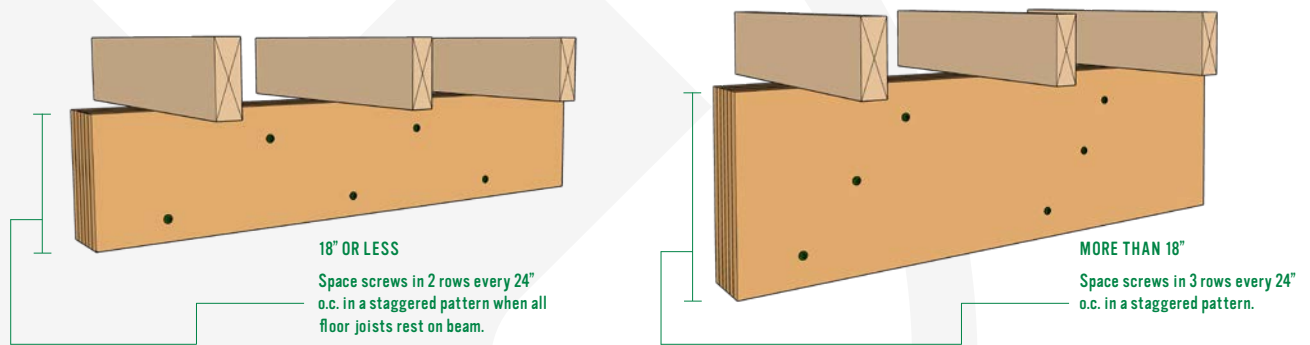
Figure 5 : Top Loaded Beams
