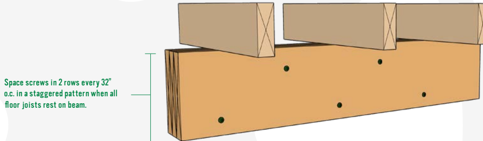
Figure 4: SPAX® 5/16" Powerlag® Fastener Assemblies for Truss and Sawn Lumber
